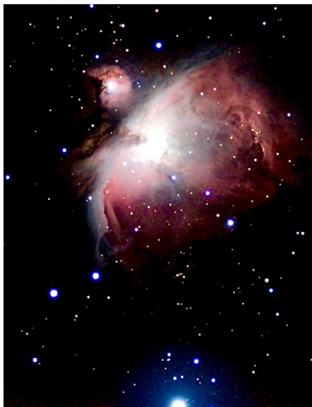
The Great Nebula in Orion
